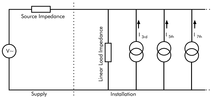
Figure 11 - Equivalent circuit of a non-linear load
