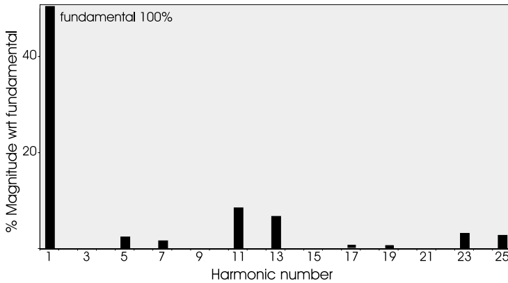
Figure 8 - Harmonic spectrum of a typical 12 pulse bridge
